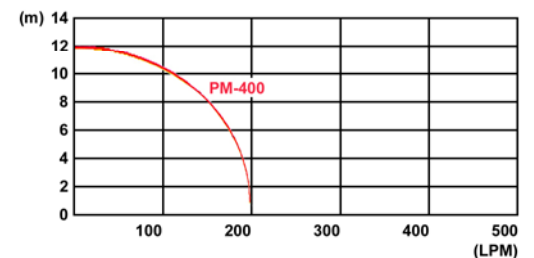
Performance Curve
